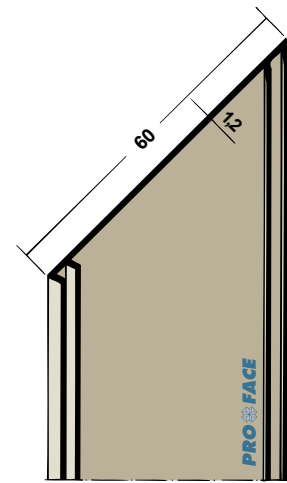
Proface®-YOIN-FLEX FL600M-P
